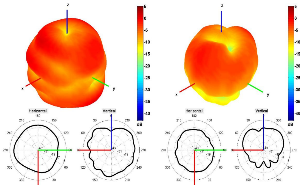
750 and 2500 MHz Radiation pattern
