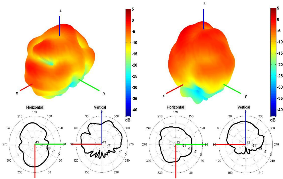
4500 and 5500 MHz Radiation pattern
