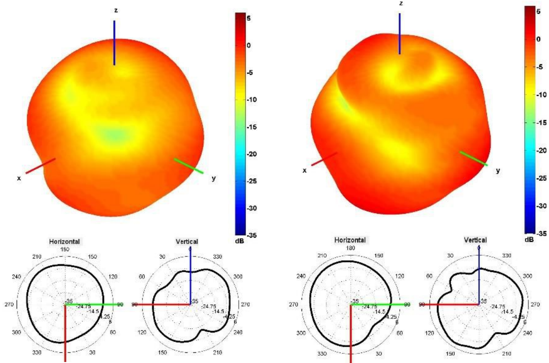
740 and 840 MHz Radiation pattern
