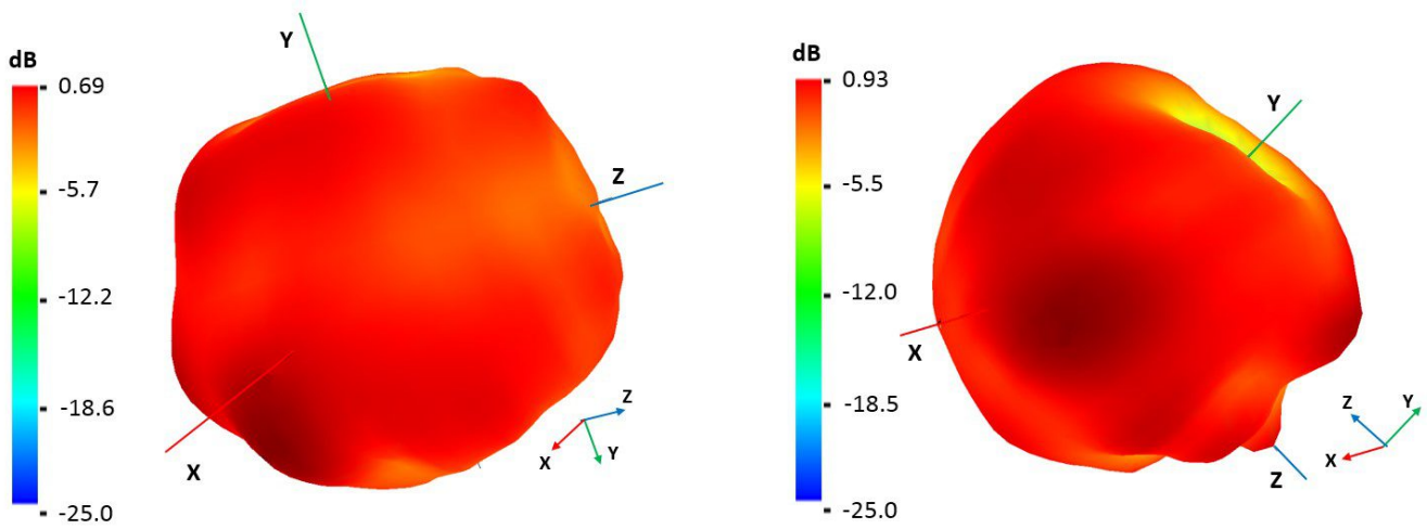
1950 and 2100 MHz Radiation pattern
