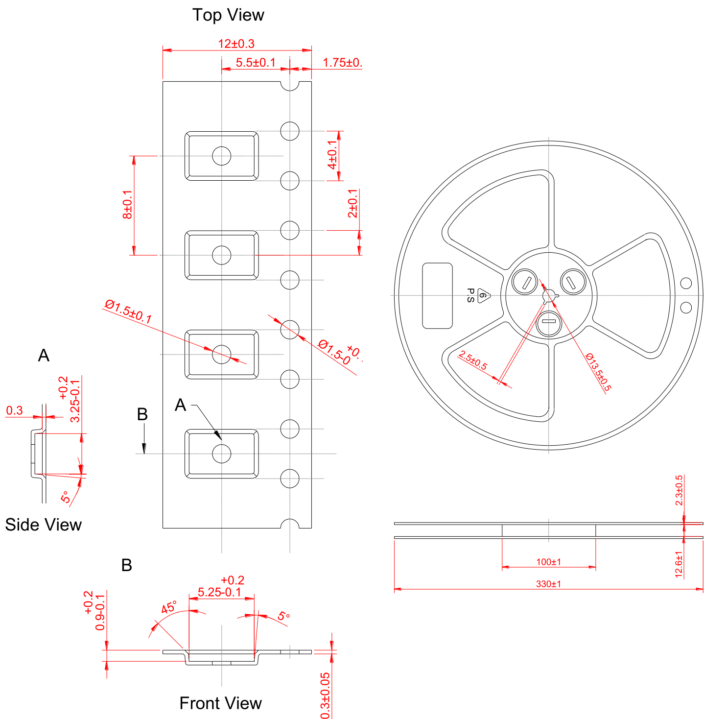
Tape and Reel Specifications
