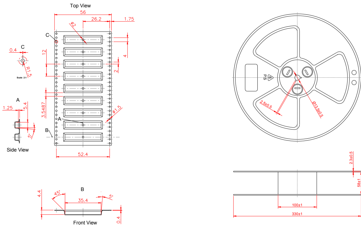
Tape and Reel Specifications
