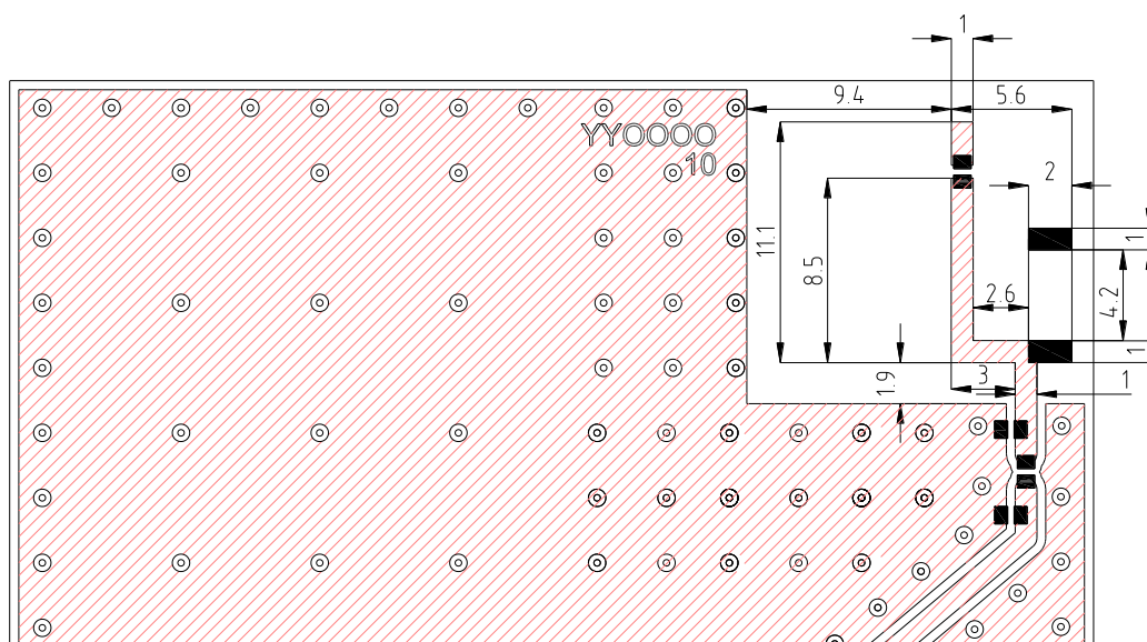
Layout dimensions for antenna integration (mm)
