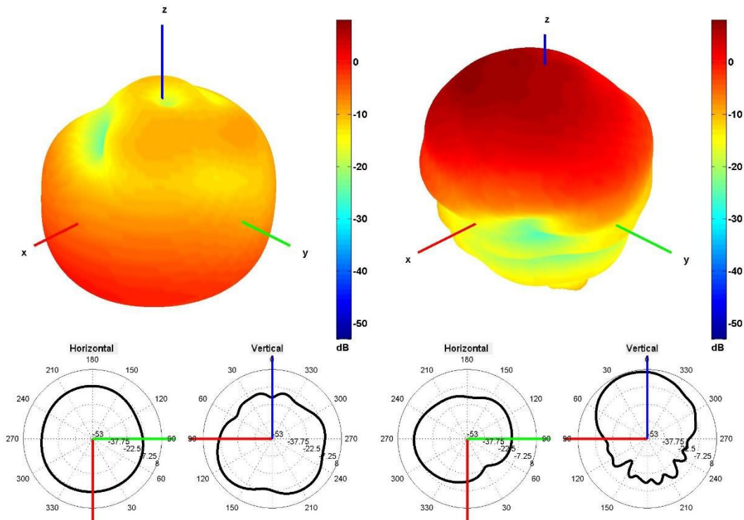
650 and 2500 MHz Radiation pattern
