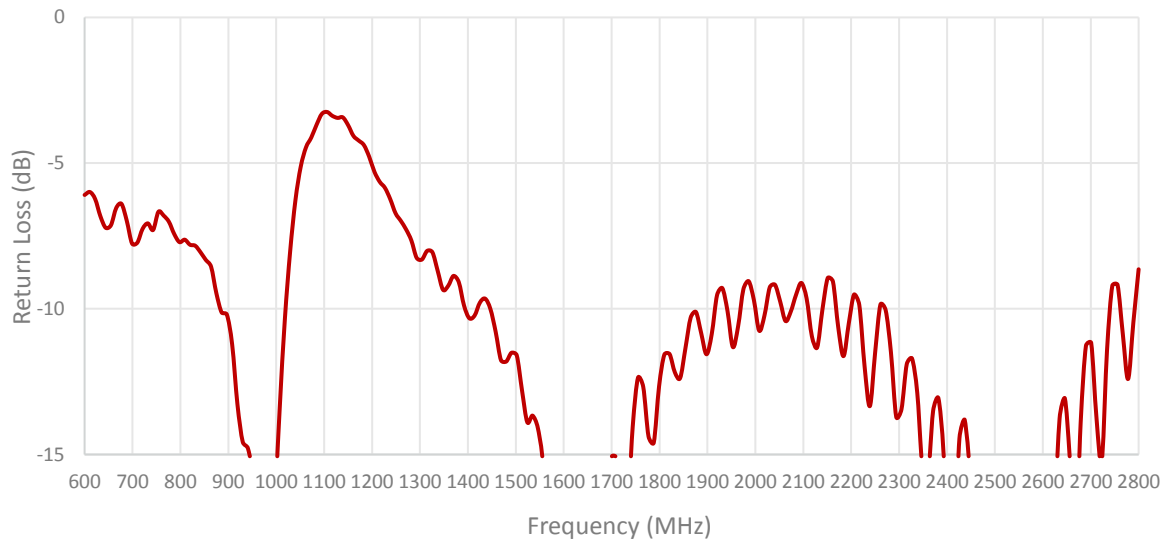
Cable 1: CELLULAR/LTE
