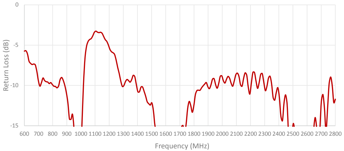
Cable 1: CELLULAR/LTE
