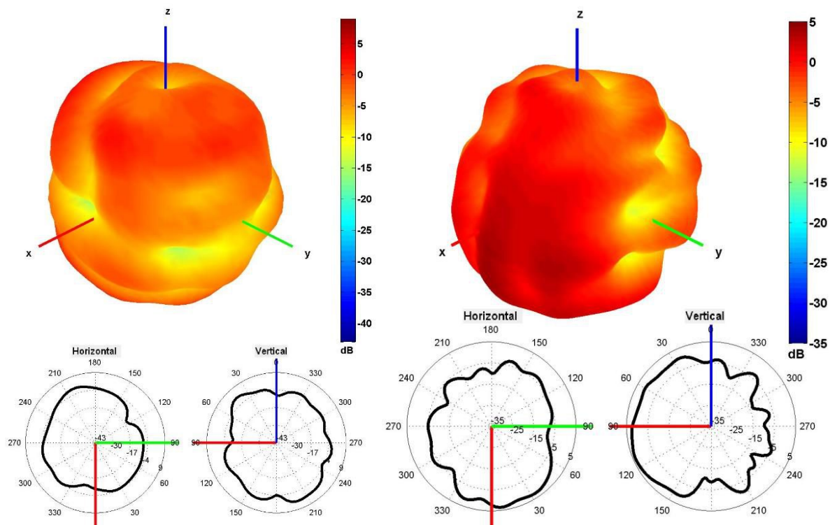
750 and 2500 MHz Radiation pattern
